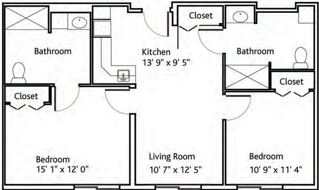
2 BEDROOM, 2 BATHROOM 830 SQUARE FEET
